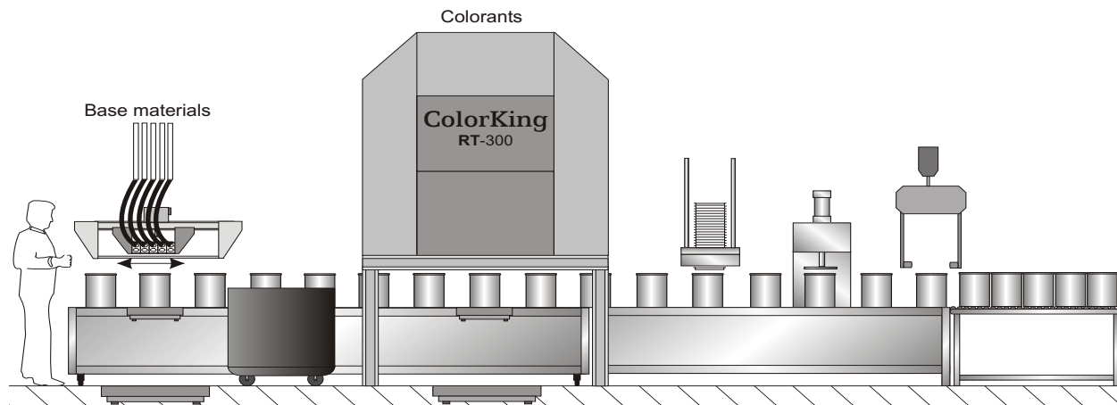
Automatic "In-can" tinting line. Also suitable for tote-dispensing.
