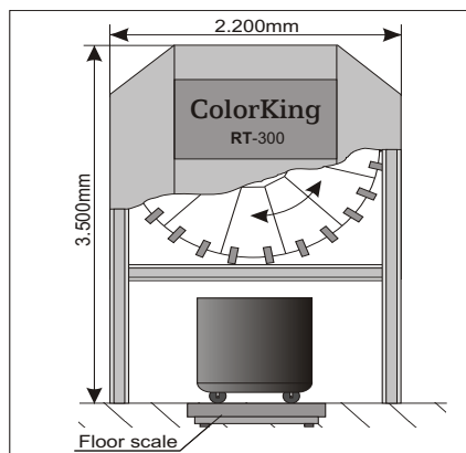
Batch dispensing
