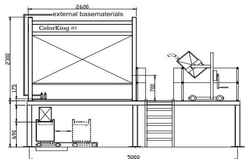
Elevated set-up. ColorKing RT-300. Suitable for tote-dispensing as well as "In-can" tinting. Available with container step-conveyor.
