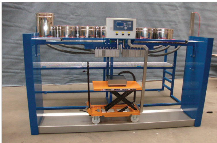
GemiTint ED-14 dispensing system. A low cost manual or semi-automatic dispenser with manual valve positioning system. The above system has 14 dispensing valves.
