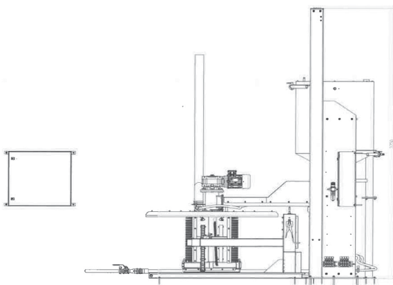
SIDE VIEW #1
