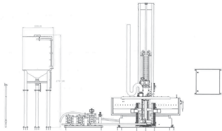
SIDE VIEW #2
