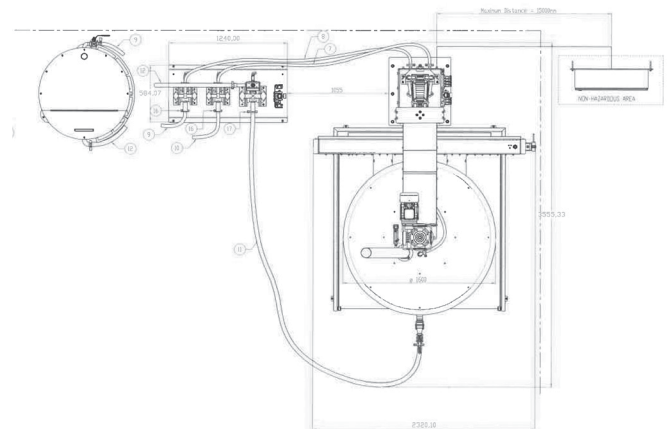
TOP VIEW #1
